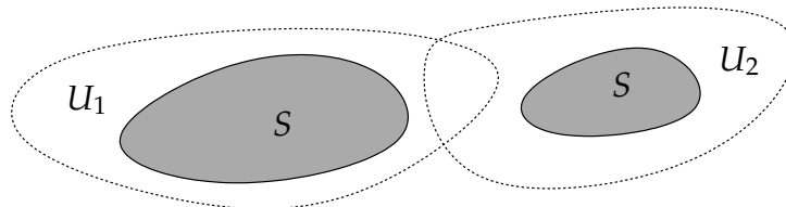
Figure 7.7: Disconnected subset. Notice that U_1 \cap U_2 need not be empty, but U_1 \cap U_2 \cap S = \emptyset .
