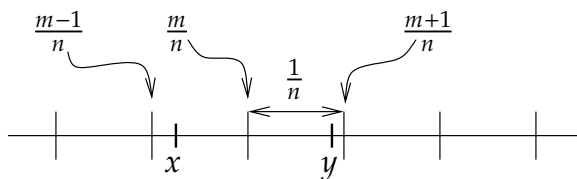
Figure 1.2: Idea of the proof of the density of \mathbb{Q} : Find n such that y - x > 1/n , then take the least m such that m/n > x .
