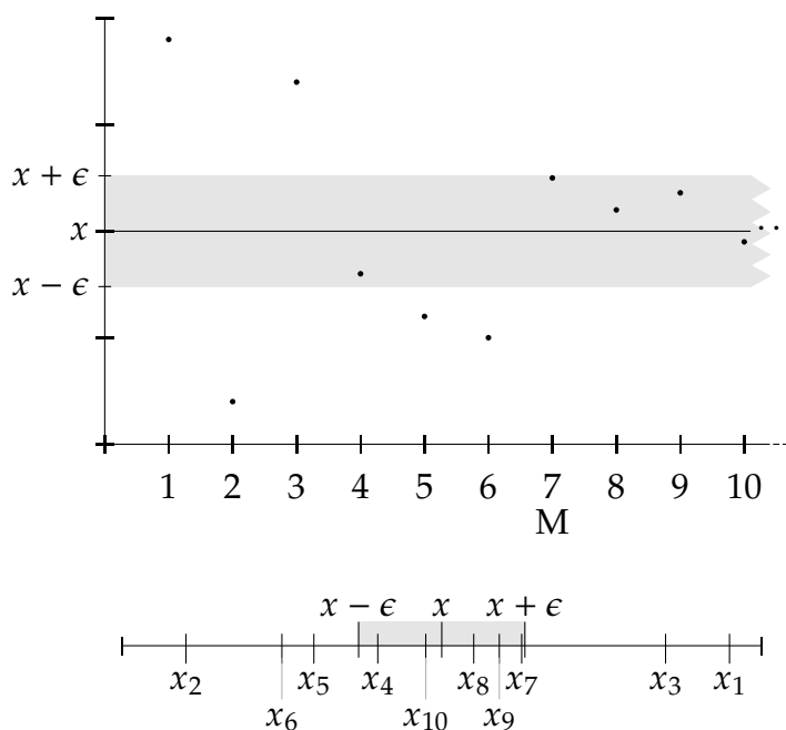
Figure 2.1: Illustration of convergence. On top, we show the first ten points of the sequence as a graph with M and the interval around the limit x marked. On bottom, the points of the same sequence are marked on the number line.
