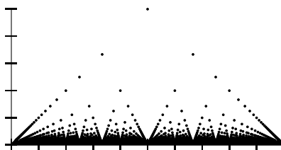
Figure 3.5: Graph of the “popcorn function.”
