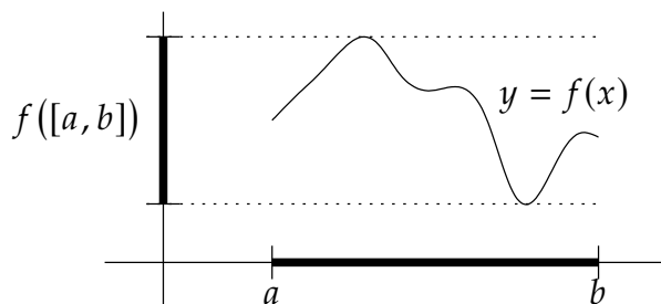
Figure 3.8: The image of a continuous f: [a, b] \rightarrow \mathbb{R} .
