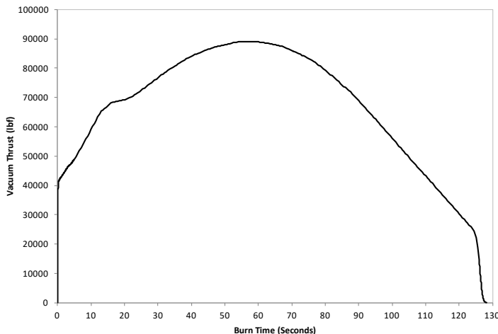
CASTOR 30B Vacuum Thrust vs. Time
